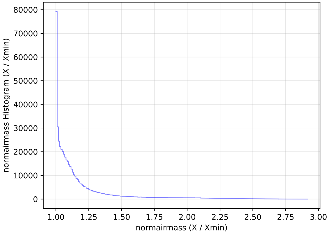
weather_cloudso35v3.4_10yrs WFD i band: normairmass Histogram
