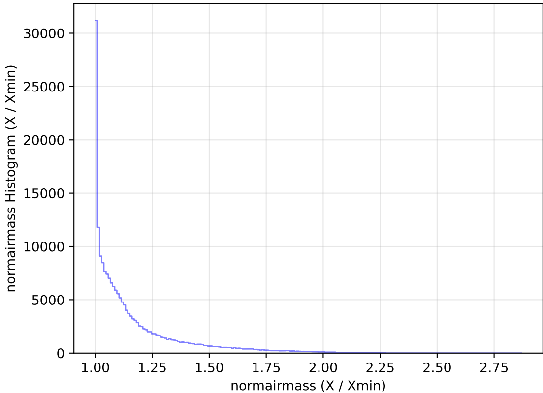
weather_cloudso35v3.4_10yrs WFD g band: normairmass Histogram
