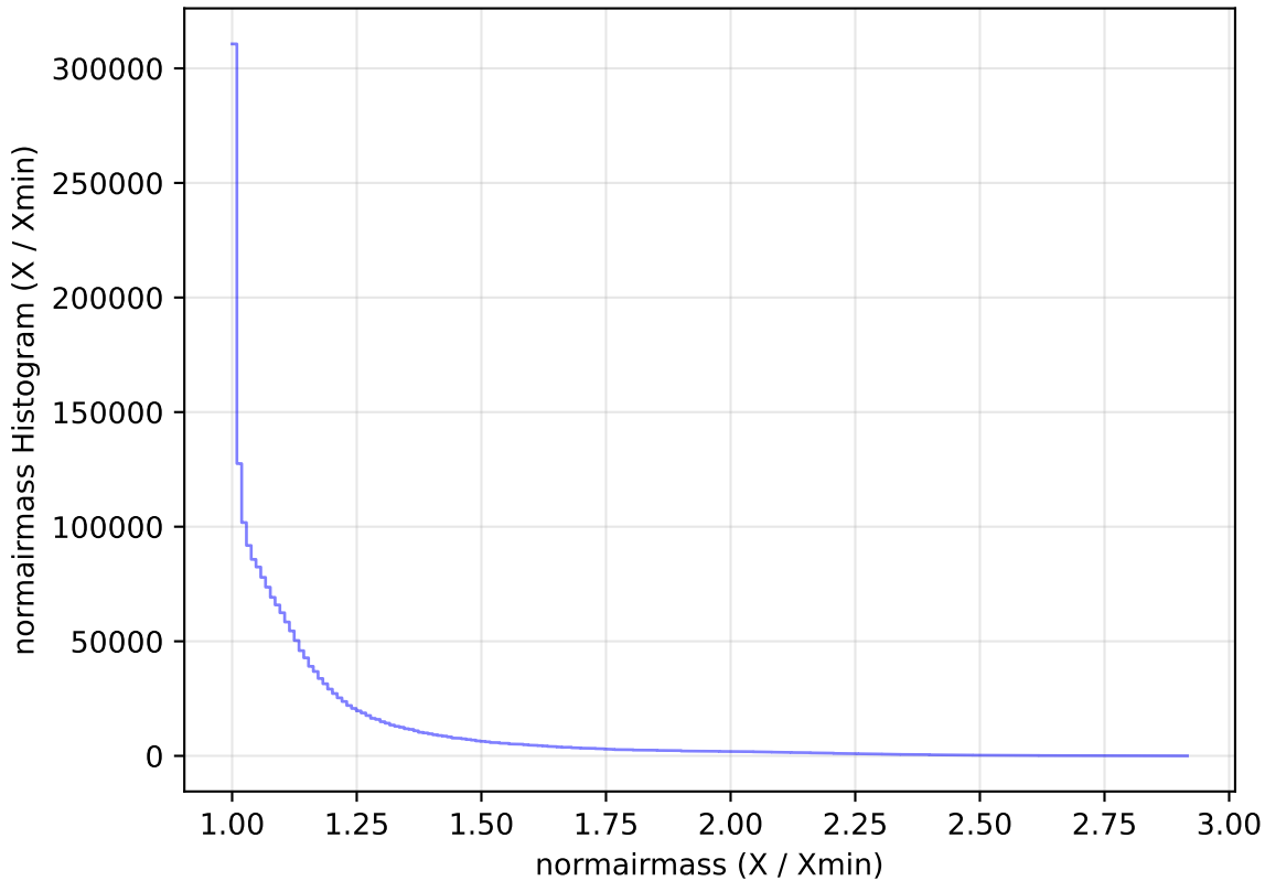
weather_cloudso35v3.4_10yrs WFD all bands: normairmass Histogram
