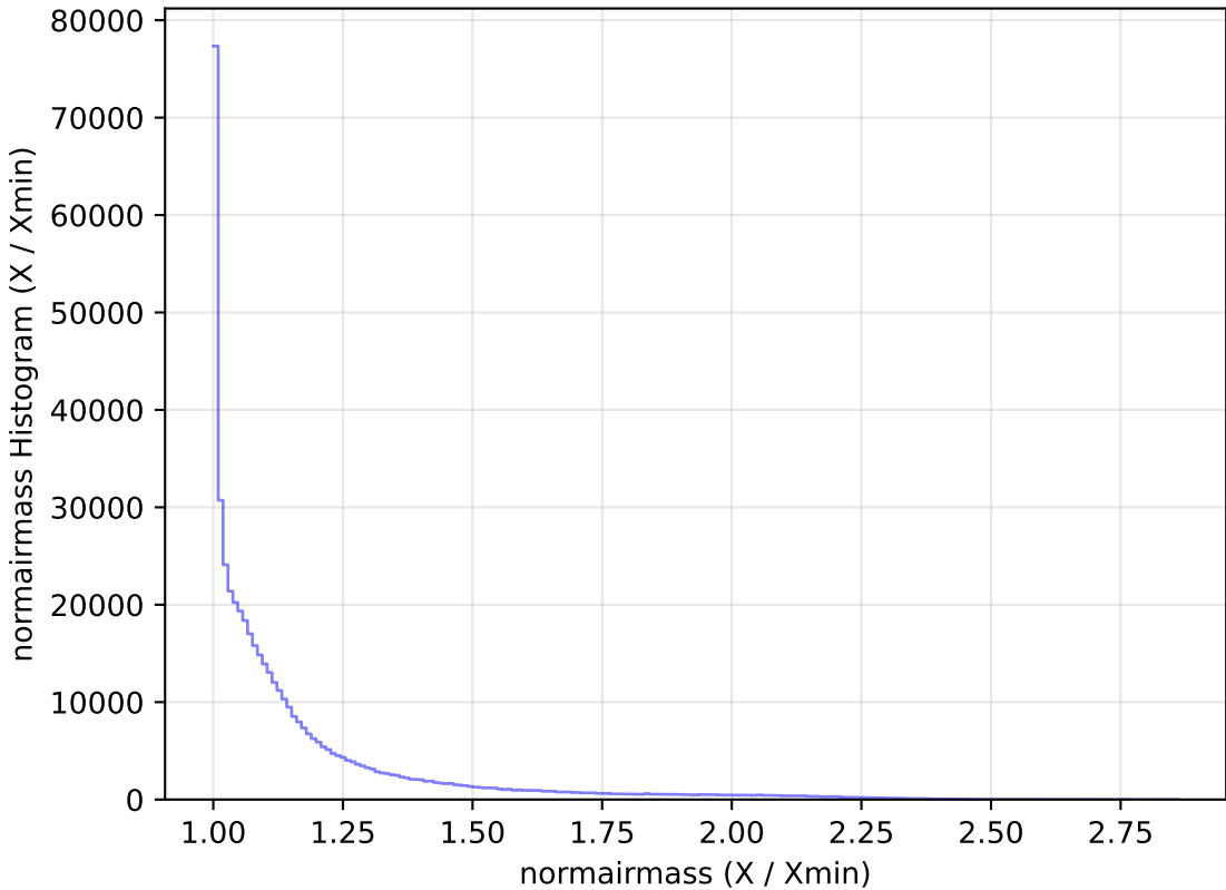
weather_cloudso35v3.4_10yrs All sky r band: normairmass Histogram
