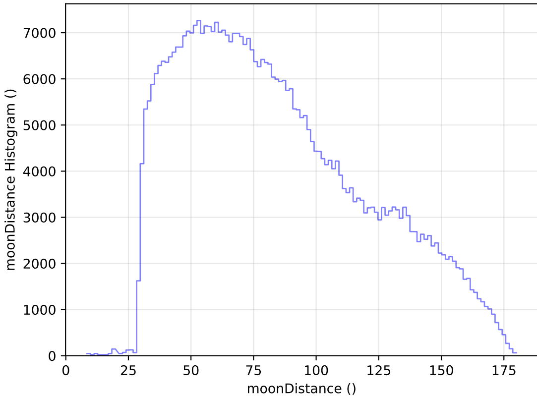
weather_cloudso35v3.4_10yrs WFD z band: moonDistance Histogram
