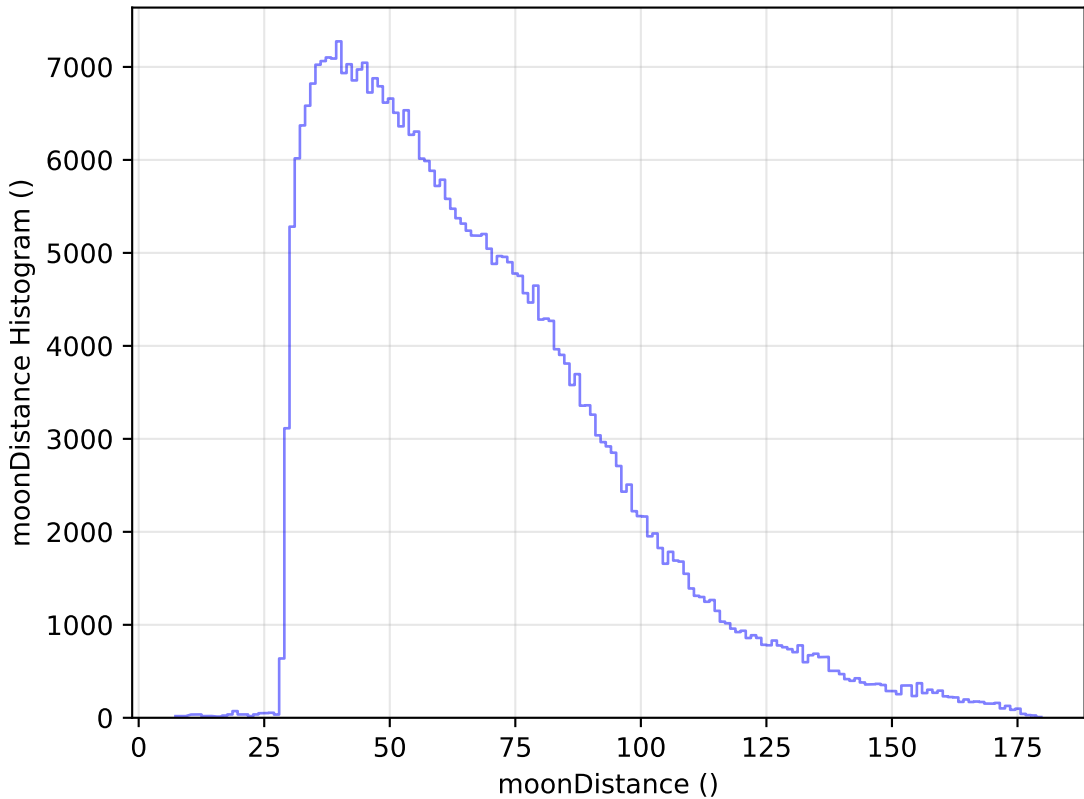
weather_cloudso35v3.4_10yrs WFD y band: moonDistance Histogram
