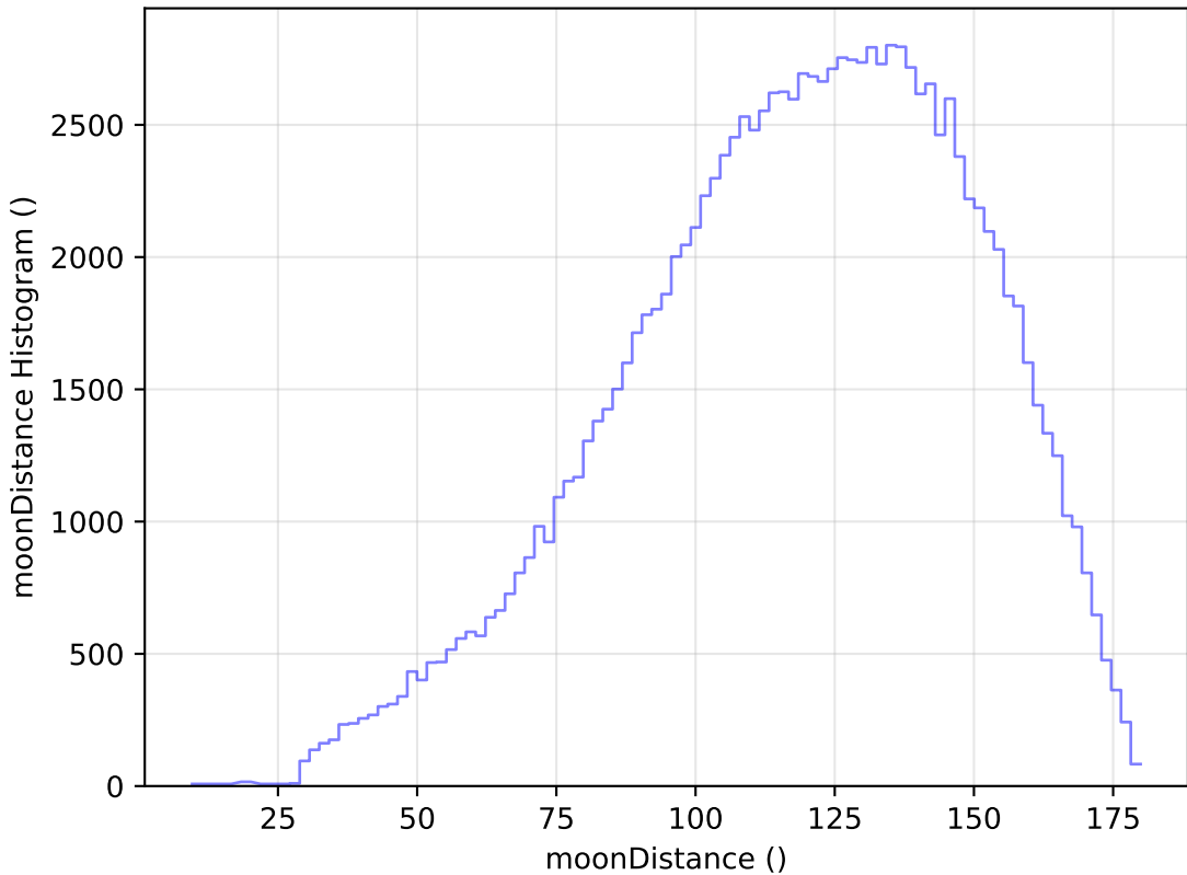
weather_cloudso35v3.4_10yrs WFD u band: moonDistance Histogram
