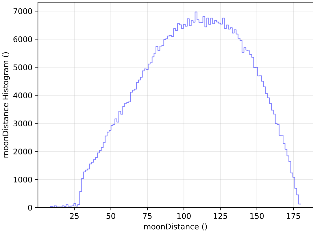
weather_cloudso35v3.4_10yrs WFD r band: moonDistance Histogram
