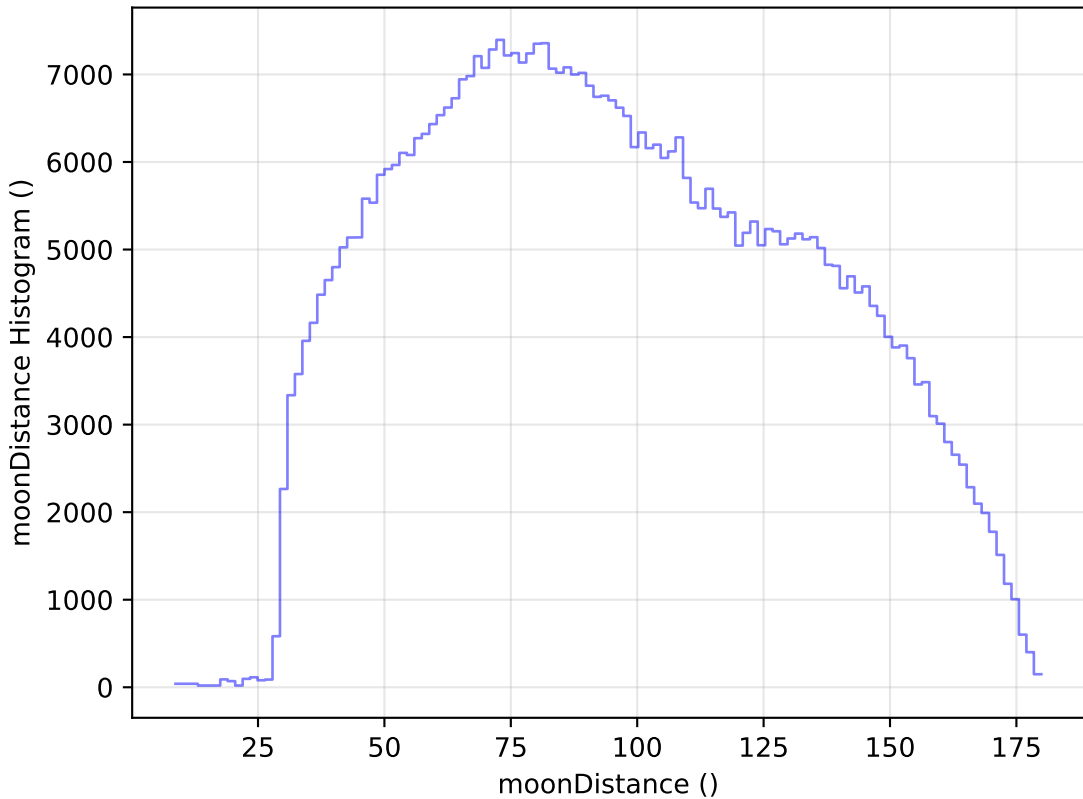
weather_cloudso35v3.4_10yrs WFD i band: moonDistance Histogram
