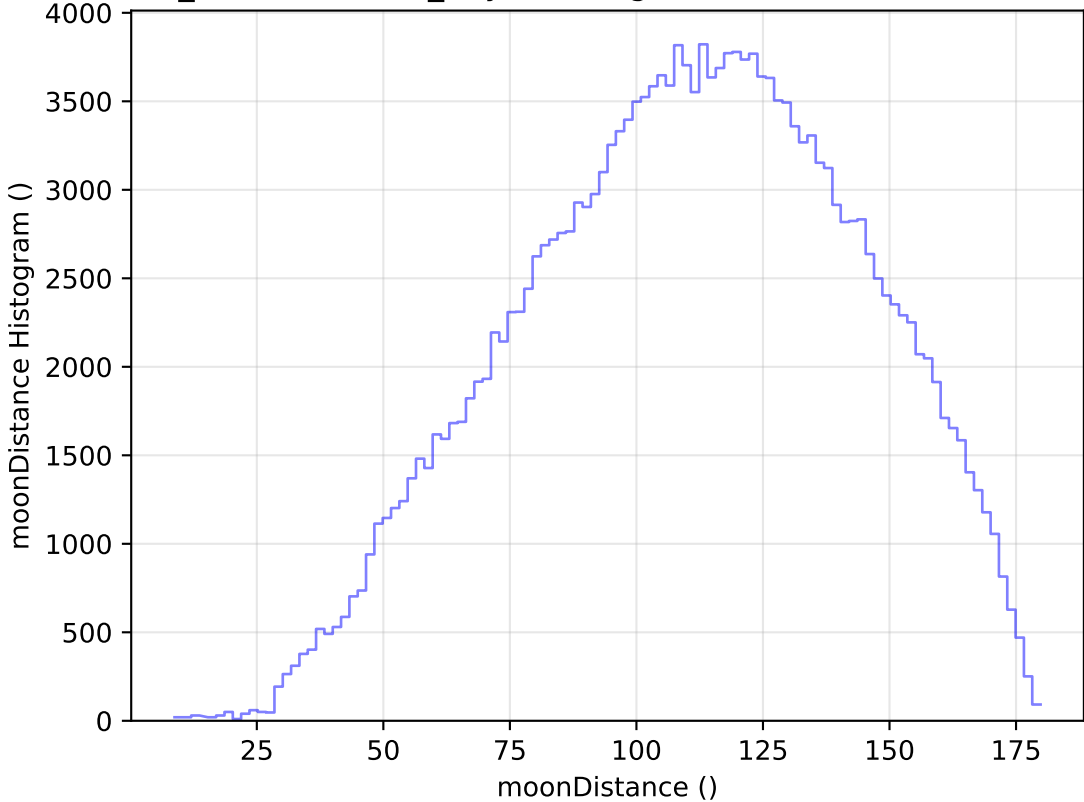
weather_cloudso35v3.4_10yrs WFD g band: moonDistance Histogram
