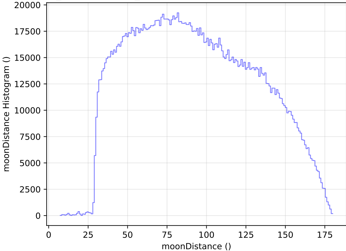
weather_cloudso35v3.4_10yrs WFD all bands: moonDistance Histogram
