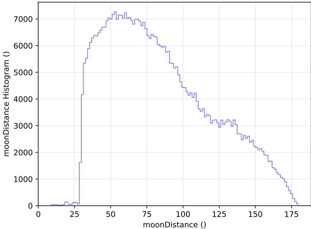
weather_cloudso35v3.4_10yrs All sky z band: moonDistance Histogram
