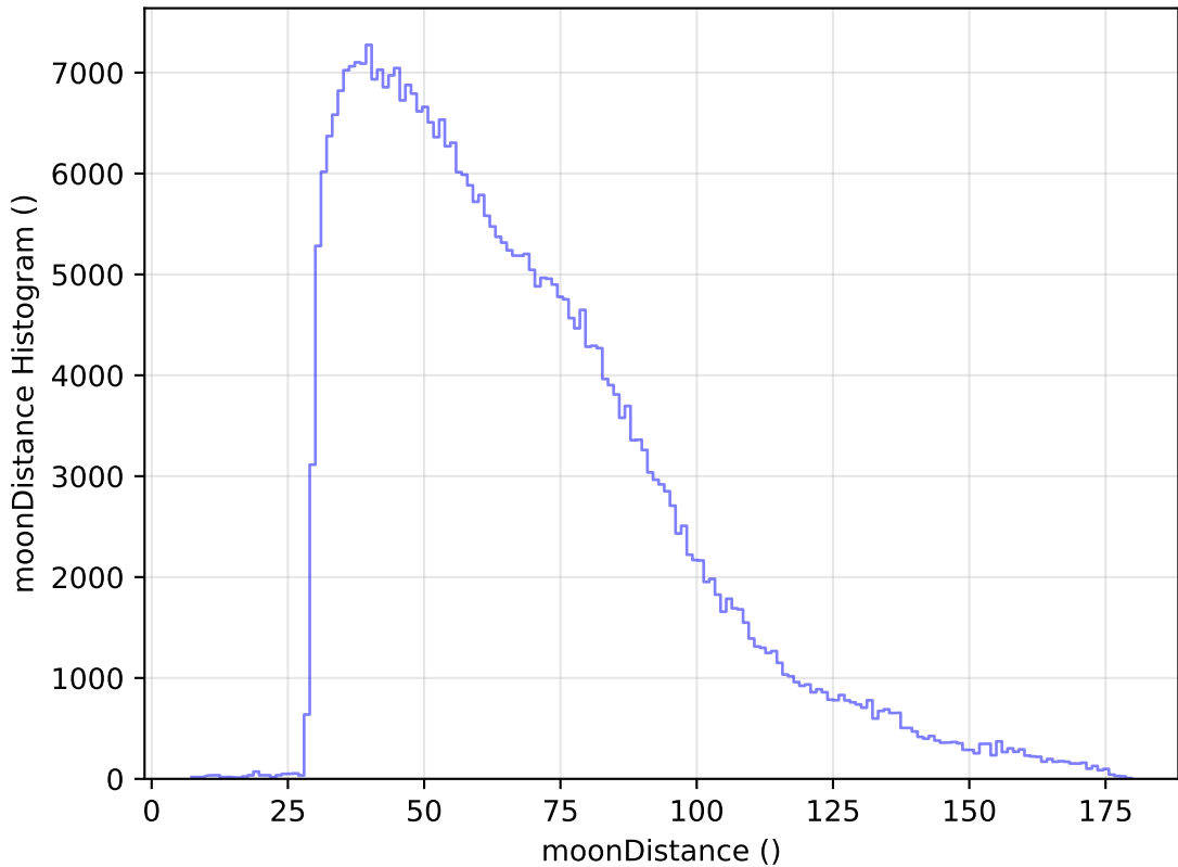
weather_cloudso35v3.4_10yrs All sky y band: moonDistance Histogram
