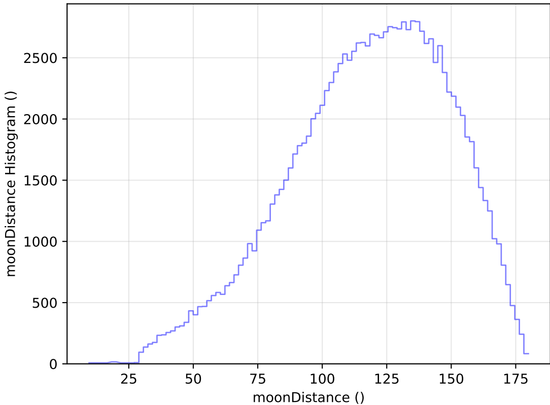
weather_cloudso35v3.4_10yrs All sky u band: moonDistance Histogram
