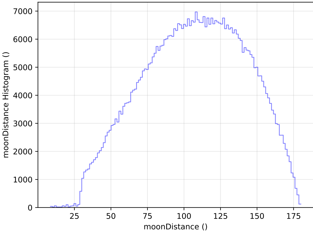
weather_cloudso35v3.4_10yrs All sky r band: moonDistance Histogram
