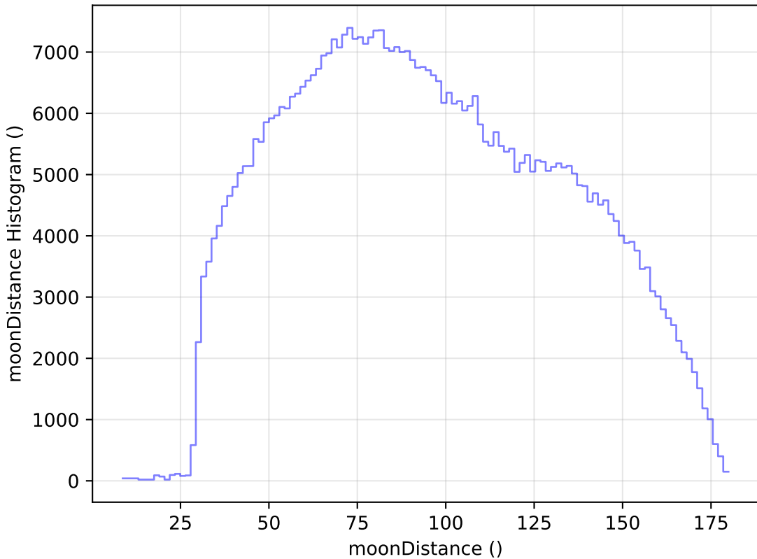
weather_cloudso35v3.4_10yrs All sky i band: moonDistance Histogram
