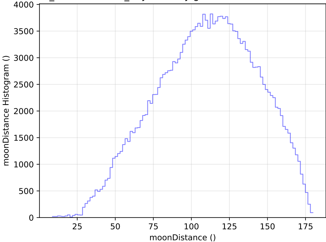
weather_cloudso35v3.4_10yrs All sky g band: moonDistance Histogram
