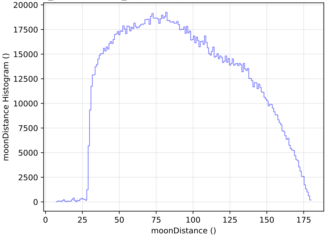
weather_cloudso35v3.4_10yrs All sky all bands: moonDistance Histogram
