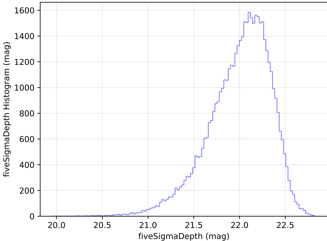
weather_cloudso35v3.4_10yrs Yr 1 y band: fiveSigmaDepth Histogram
