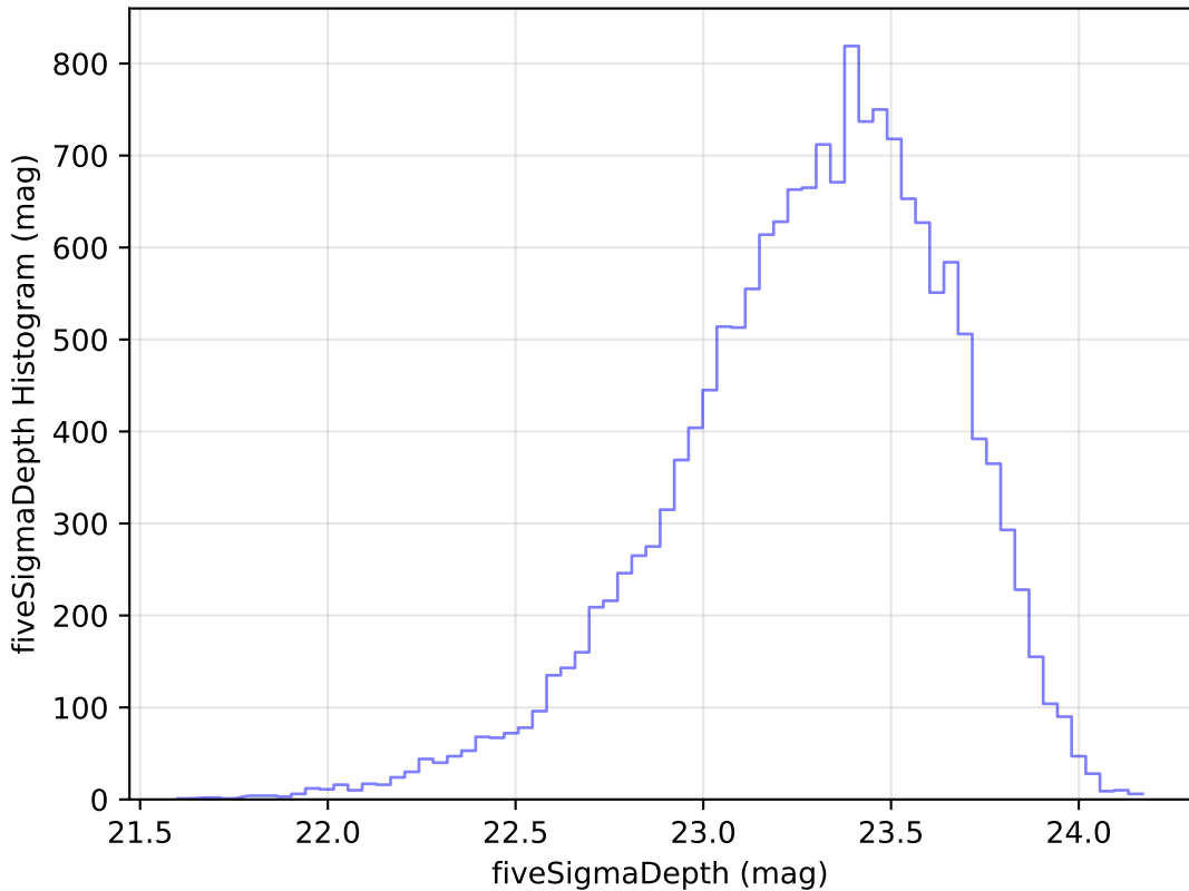
weather_cloudso35v3.4_10yrs Yr 1 u band: fiveSigmaDepth Histogram
