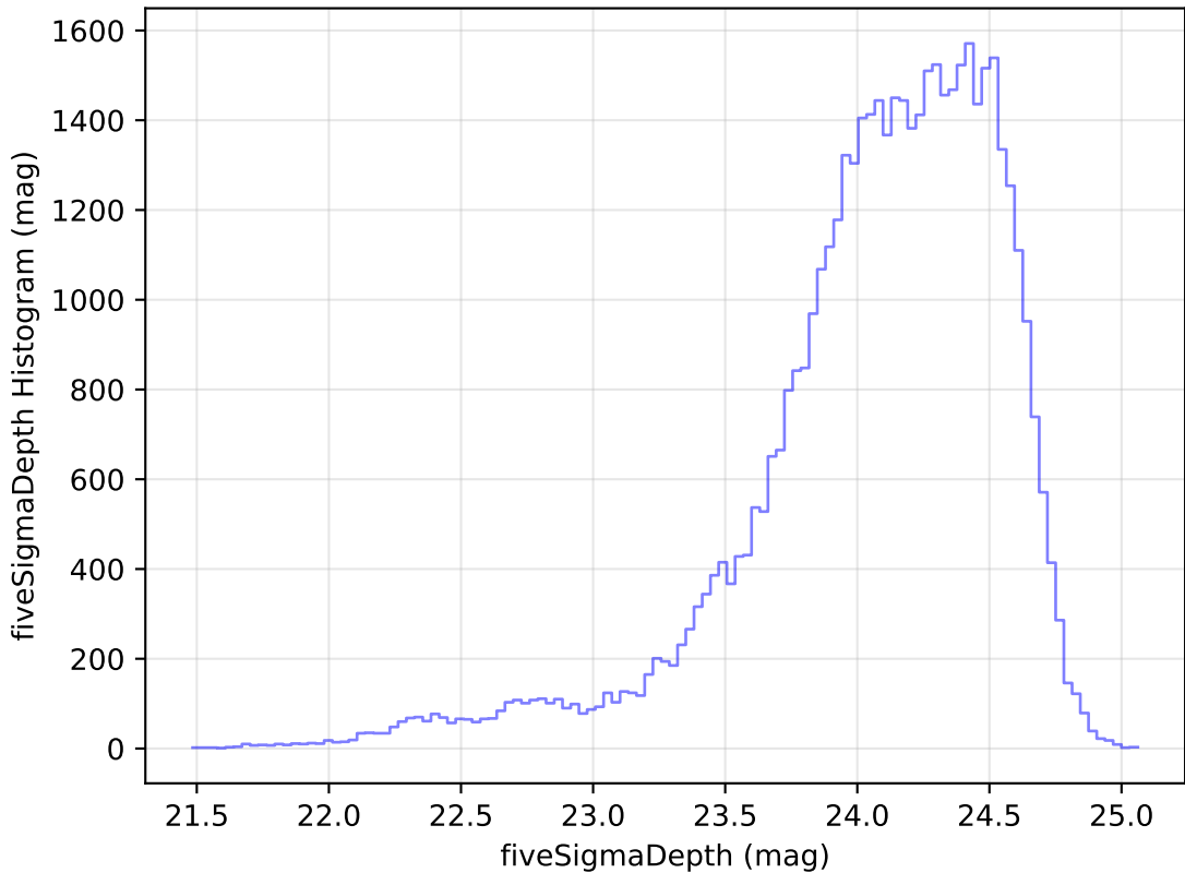
weather_cloudso35v3.4_10yrs Yr 1 r band: fiveSigmaDepth Histogram
