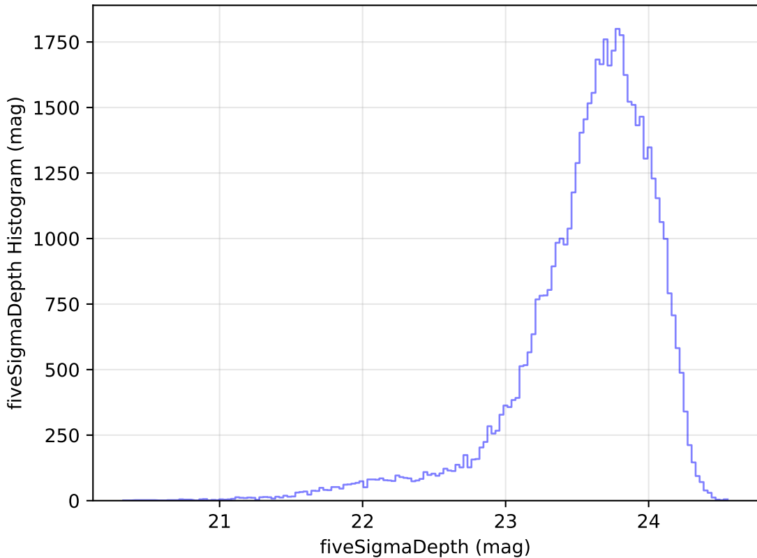
weather_cloudso35v3.4_10yrs Yr 1 i band: fiveSigmaDepth Histogram
