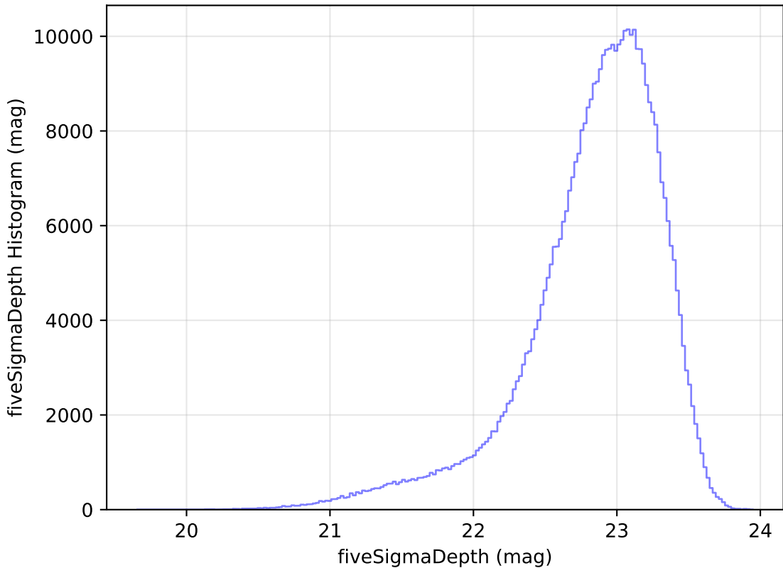
weather_cloudso35v3.4_10yrs WFD z band: fiveSigmaDepth Histogram
