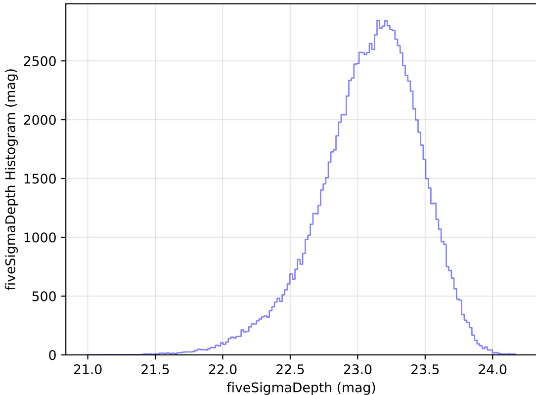
weather_cloudso35v3.4_10yrs WFD u band: fiveSigmaDepth Histogram
