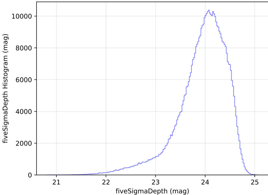
weather_cloudso35v3.4_10yrs WFD r band: fiveSigmaDepth Histogram
