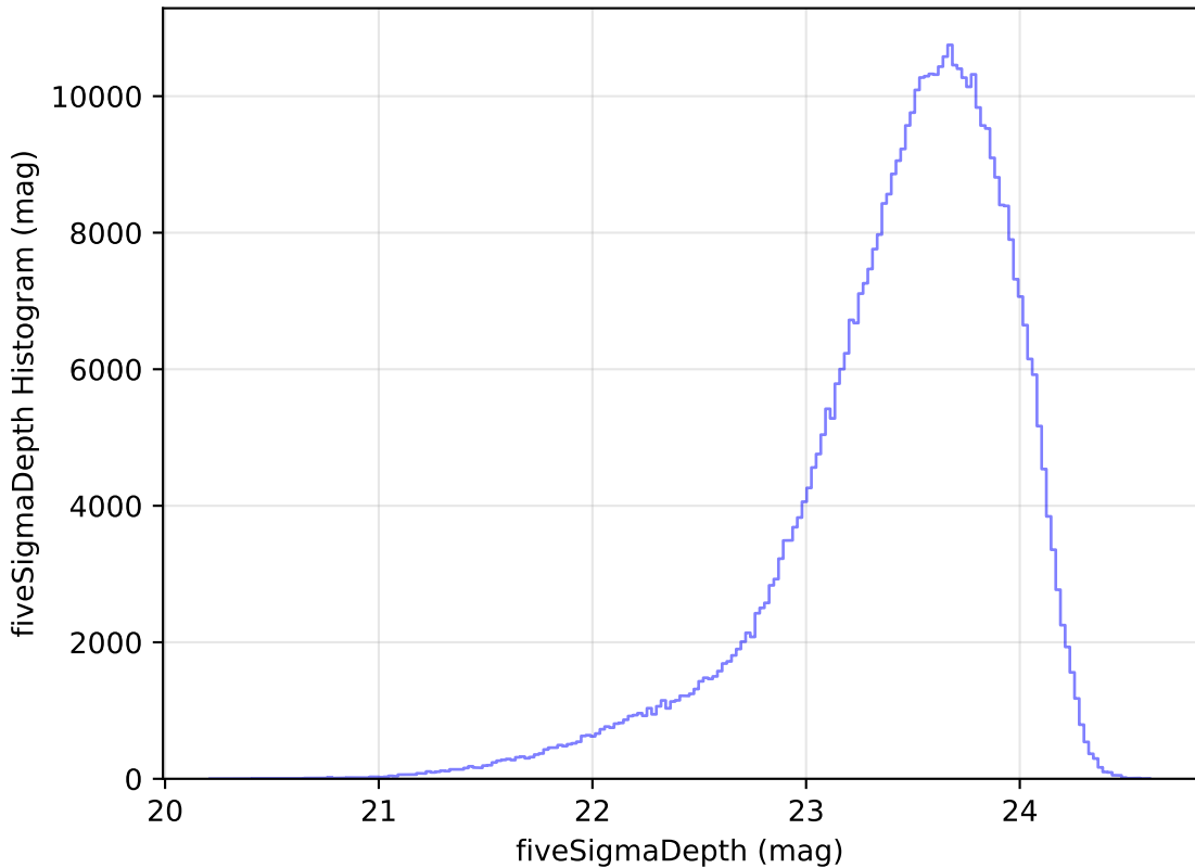
weather_cloudso35v3.4_10yrs WFD i band: fiveSigmaDepth Histogram
