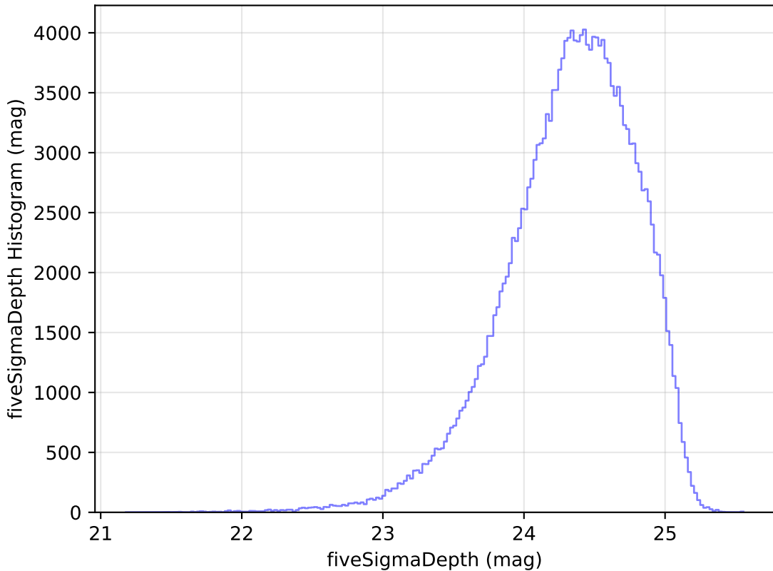
weather_cloudso35v3.4_10yrs WFD g band: fiveSigmaDepth Histogram
