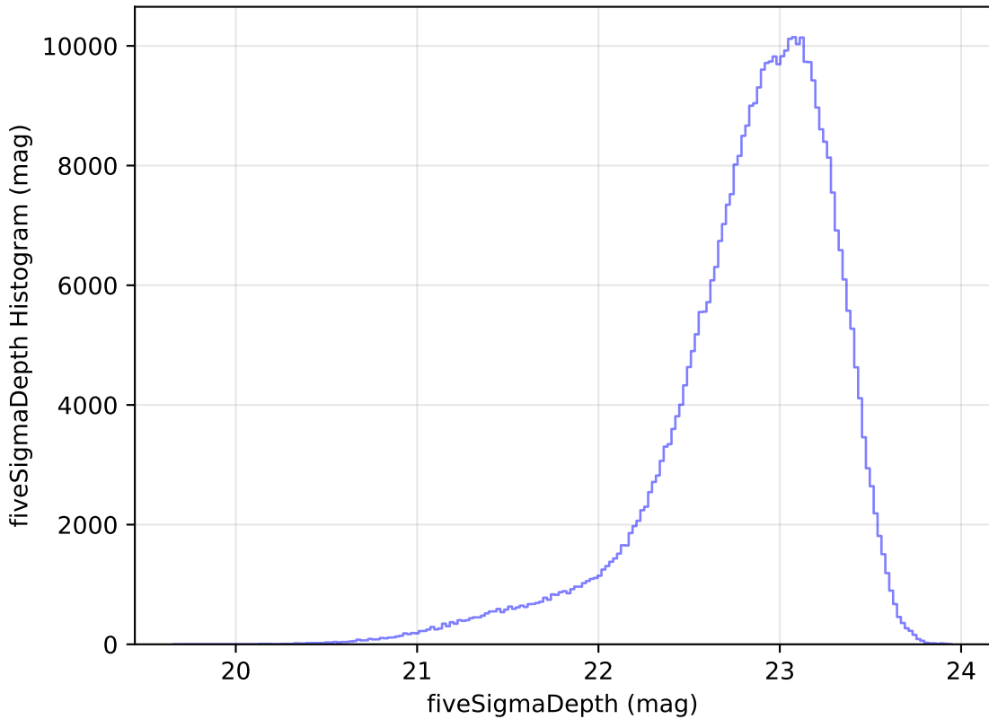
weather_cloudso35v3.4_10yrs All sky z band: fiveSigmaDepth Histogram
