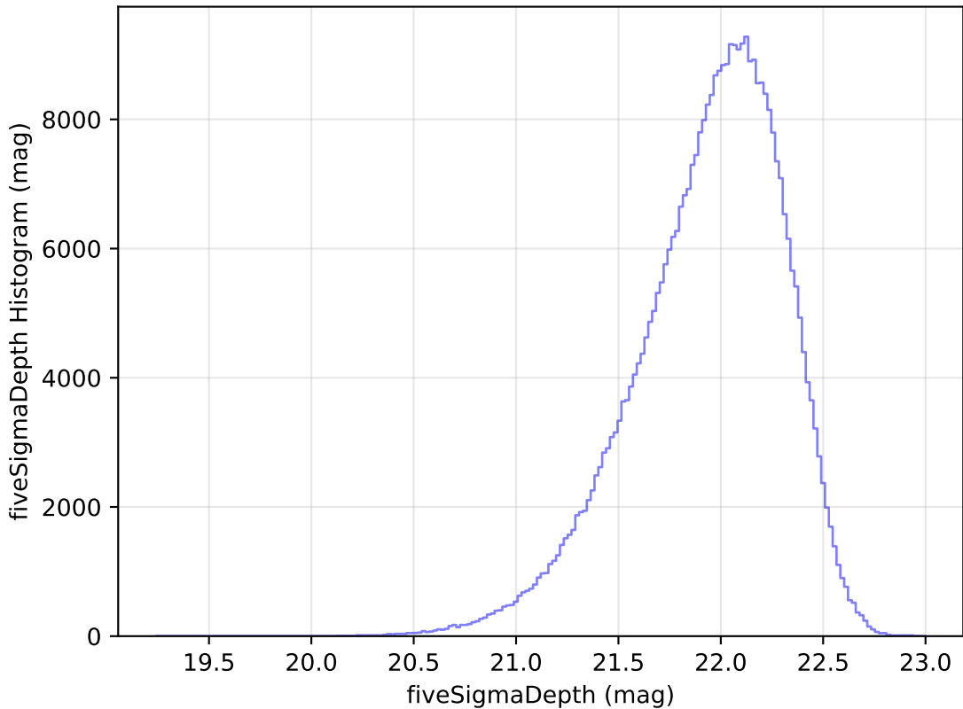
weather_cloudso35v3.4_10yrs All sky y band: fiveSigmaDepth Histogram
