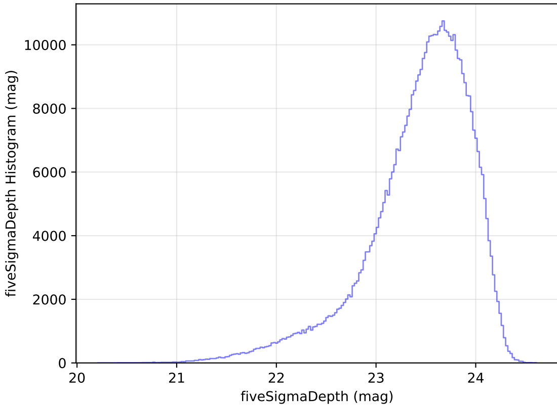
weather_cloudso35v3.4_10yrs All sky i band: fiveSigmaDepth Histogram
