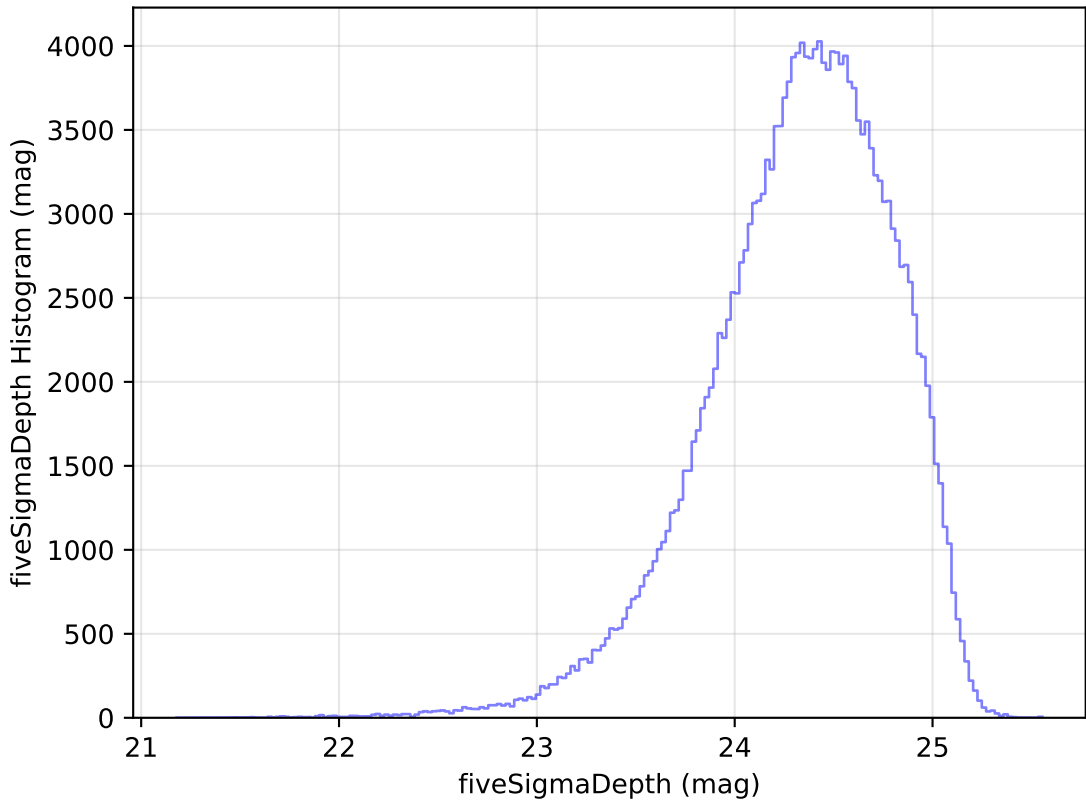
weather_cloudso35v3.4_10yrs All sky g band: fiveSigmaDepth Histogram
