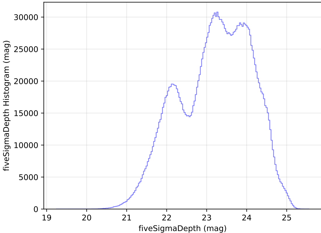
weather_cloudso35v3.4_10yrs All sky all bands: fiveSigmaDepth Histogram
