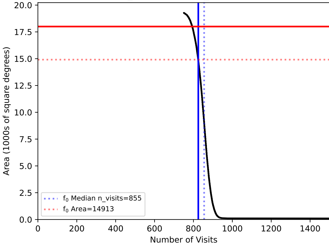
weather_cloudso35v3.4_10yrs WFD: f0
