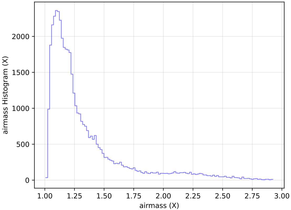
weather_cloudso35v3.4_10yrs Yr 1 z band: airmass Histogram
