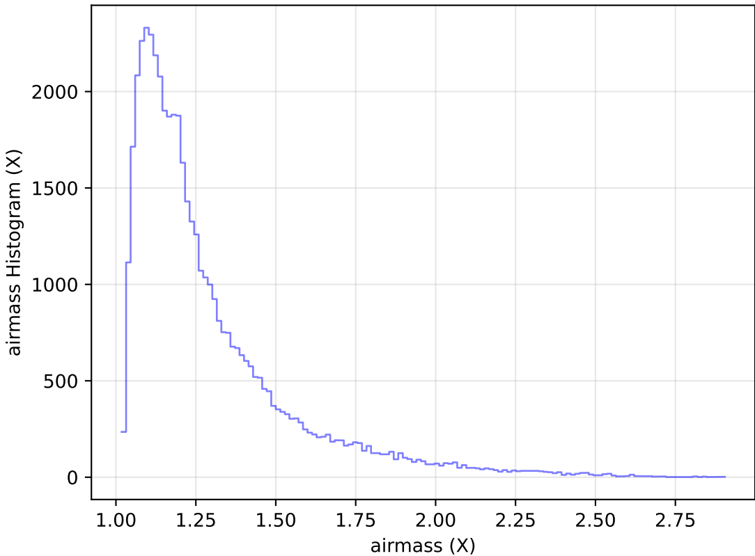
weather_cloudso35v3.4_10yrs Yr 1 y band: airmass Histogram
