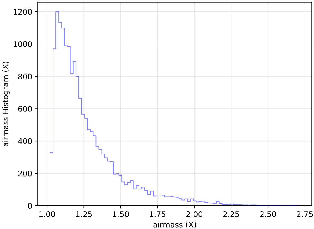
weather_cloudso35v3.4_10yrs Yr 1 u band: airmass Histogram
