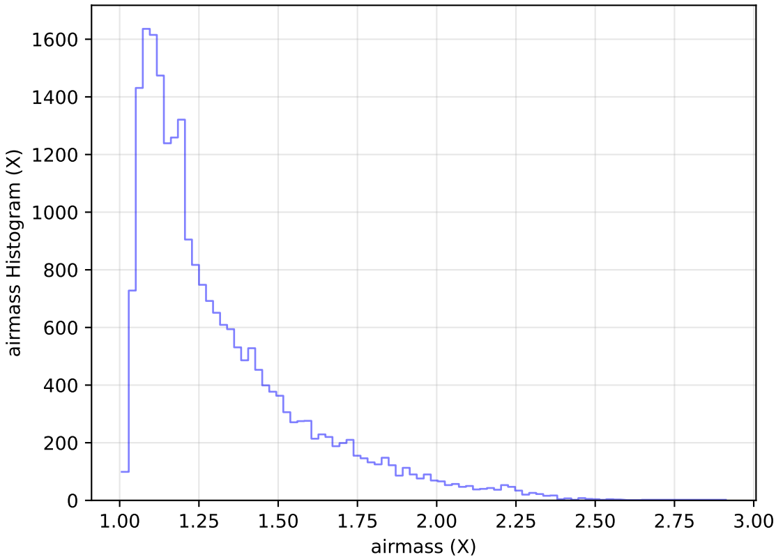
weather_cloudso35v3.4_10yrs Yr 1 g band: airmass Histogram
