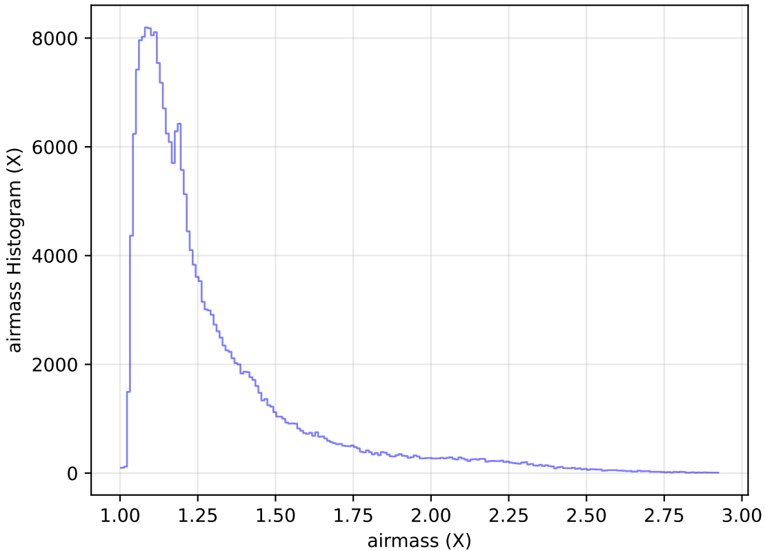
weather_cloudso35v3.4_10yrs Yr 1 all bands: airmass Histogram
