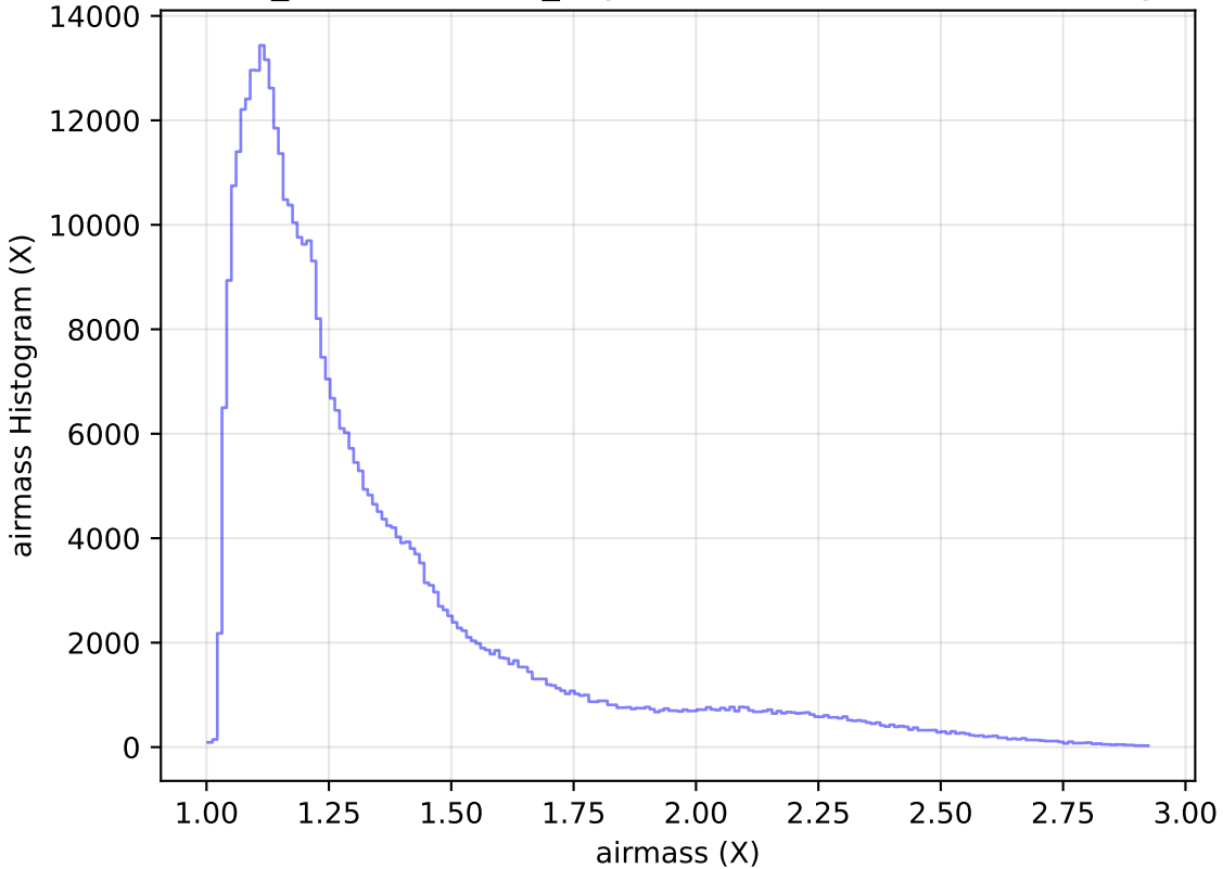
weather_cloudso35v3.4_10yrs WFD z band: airmass Histogram
