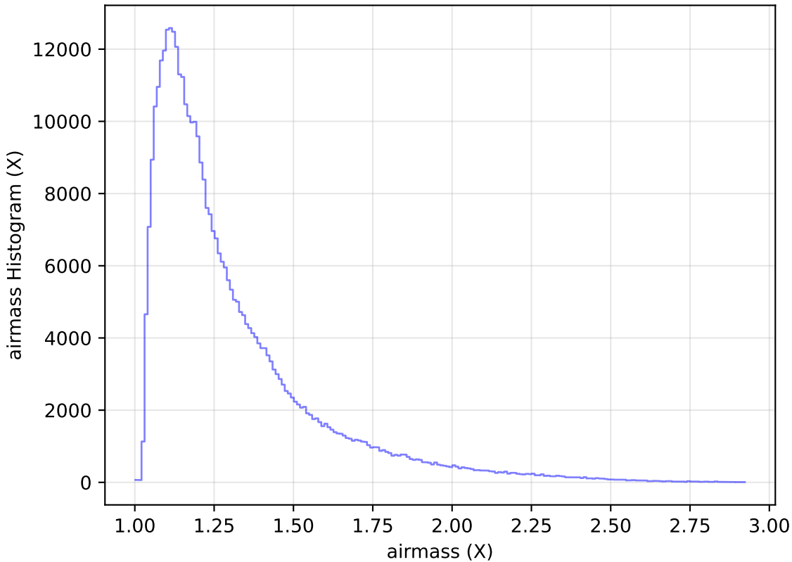
weather_cloudso35v3.4_10yrs WFD y band: airmass Histogram
