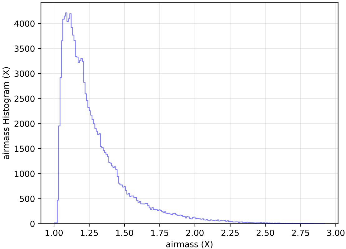
weather_cloudso35v3.4_10yrs WFD u band: airmass Histogram
