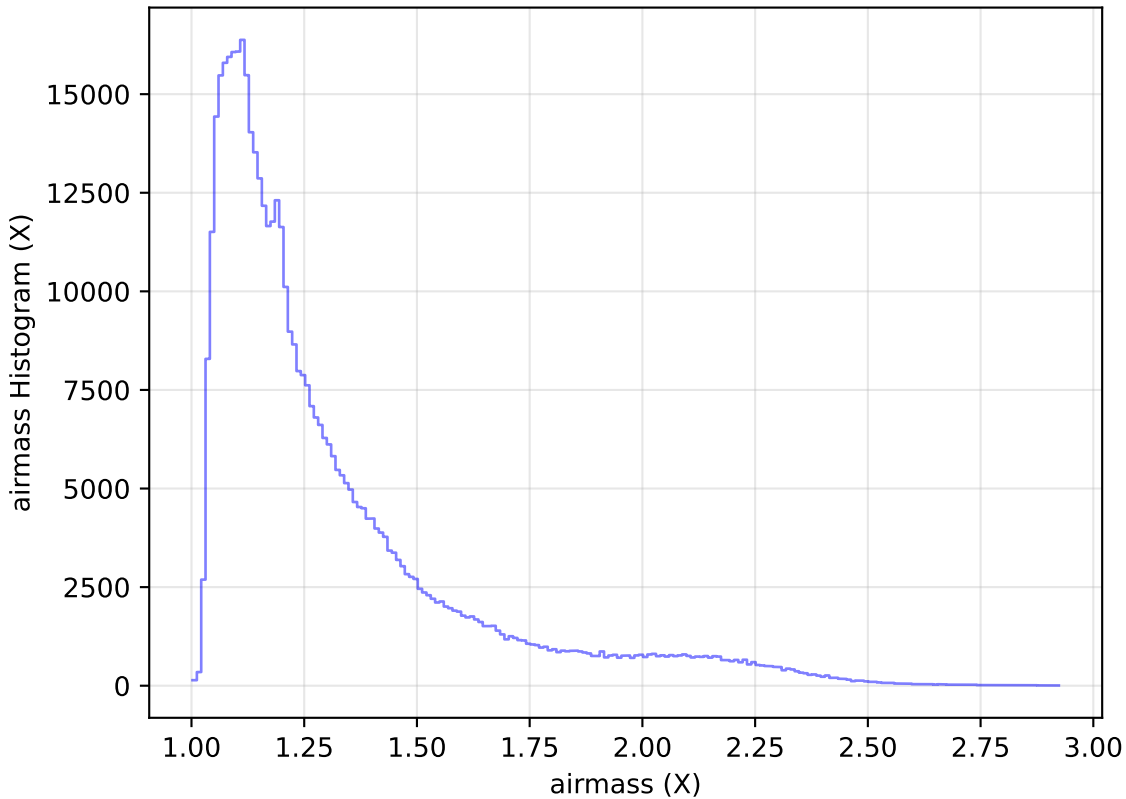
weather_cloudso35v3.4_10yrs WFD r band: airmass Histogram
