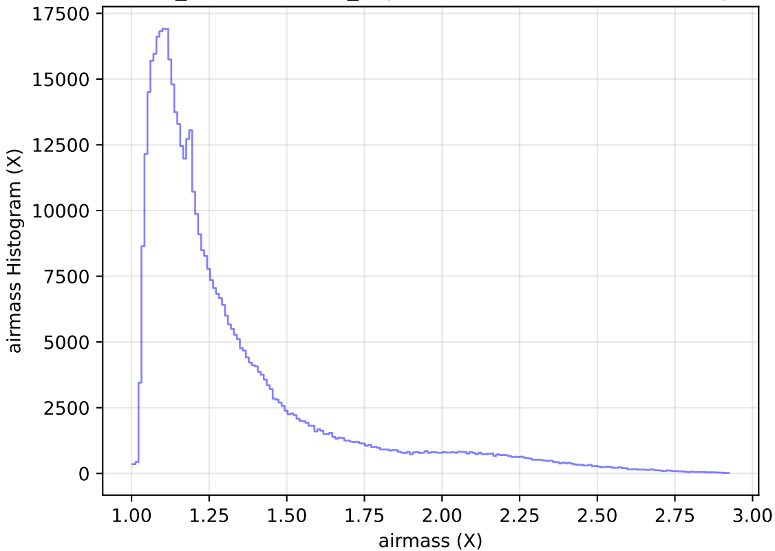
weather_cloudso35v3.4_10yrs WFD i band: airmass Histogram
