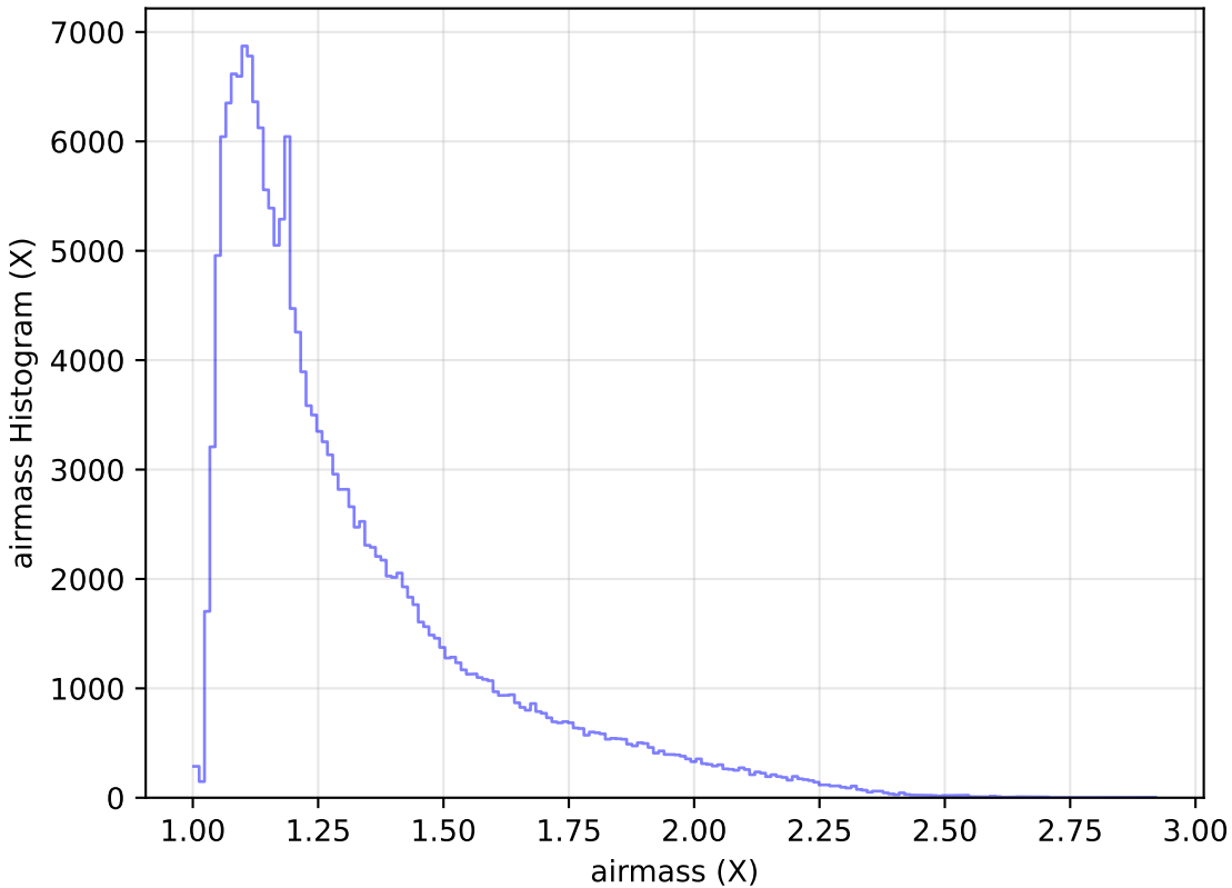
weather_cloudso35v3.4_10yrs WFD g band: airmass Histogram
