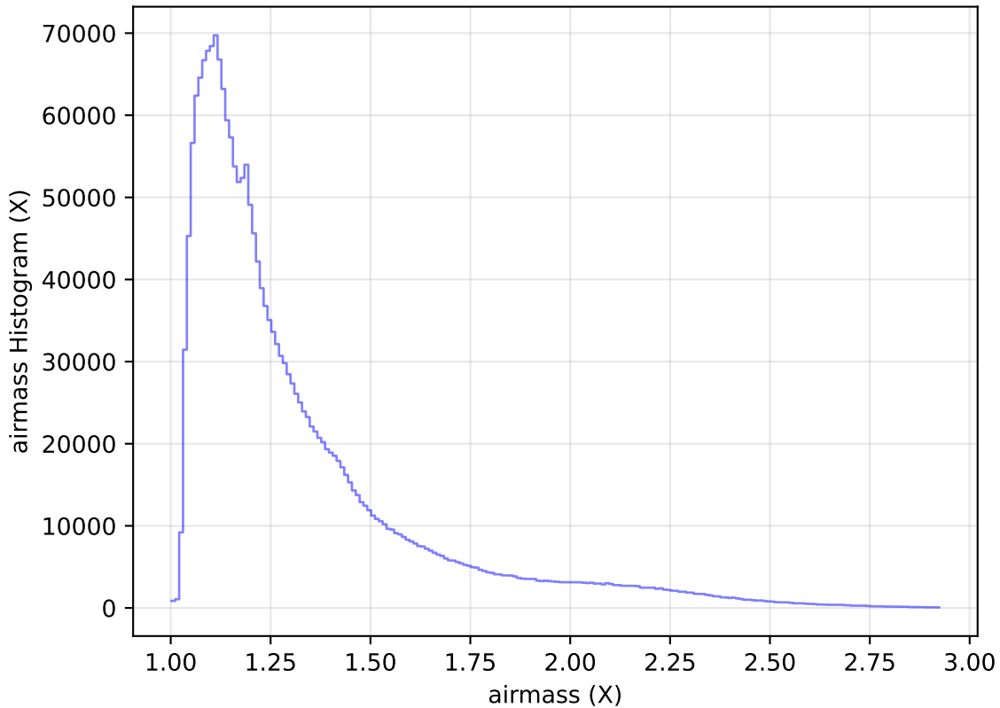
weather_cloudso35v3.4_10yrs WFD all bands: airmass Histogram
