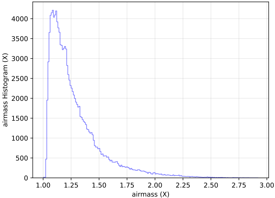
weather_cloudso35v3.4_10yrs All sky u band: airmass Histogram
