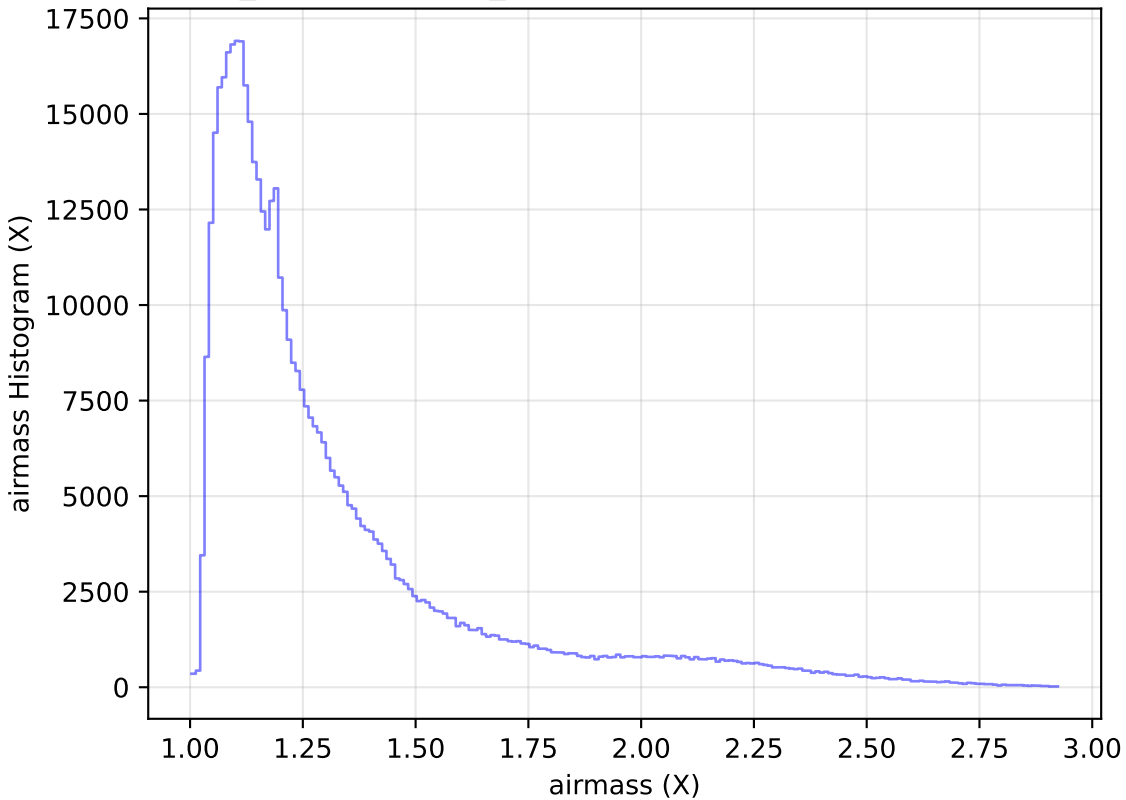
weather_cloudso35v3.4_10yrs All sky i band: airmass Histogram
