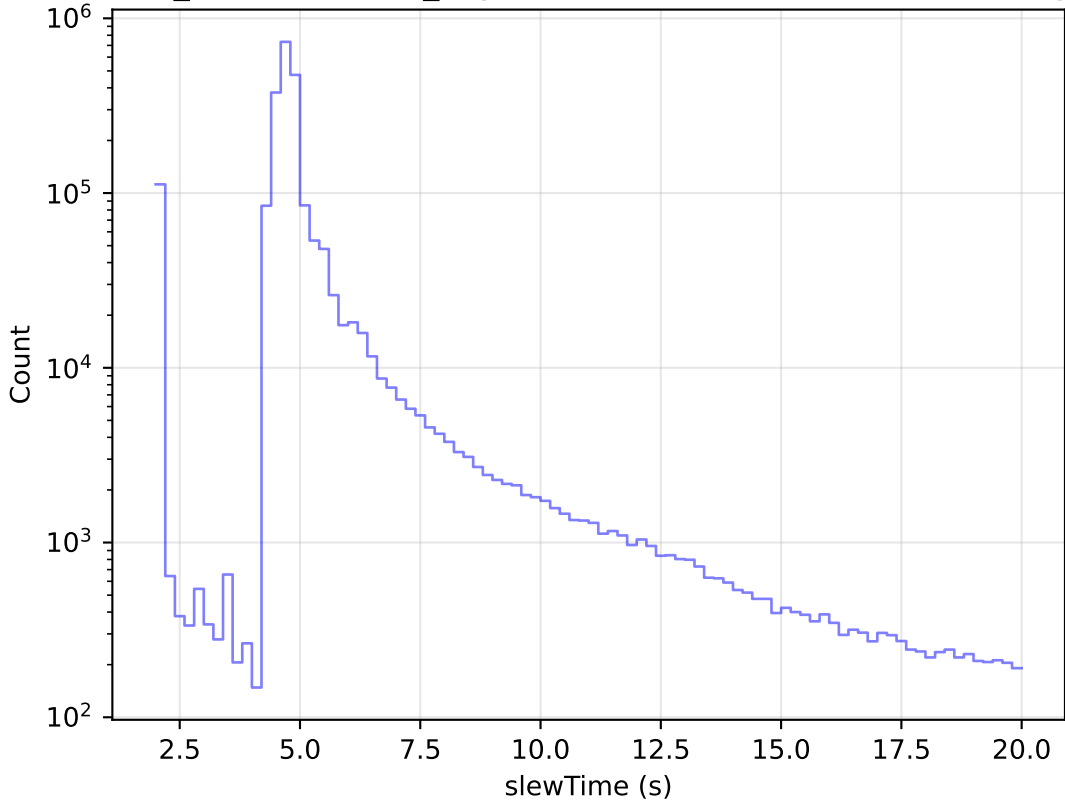
weather_cloudso35v3.4_10yrs All visits: Zoom Slew Time Histogram
