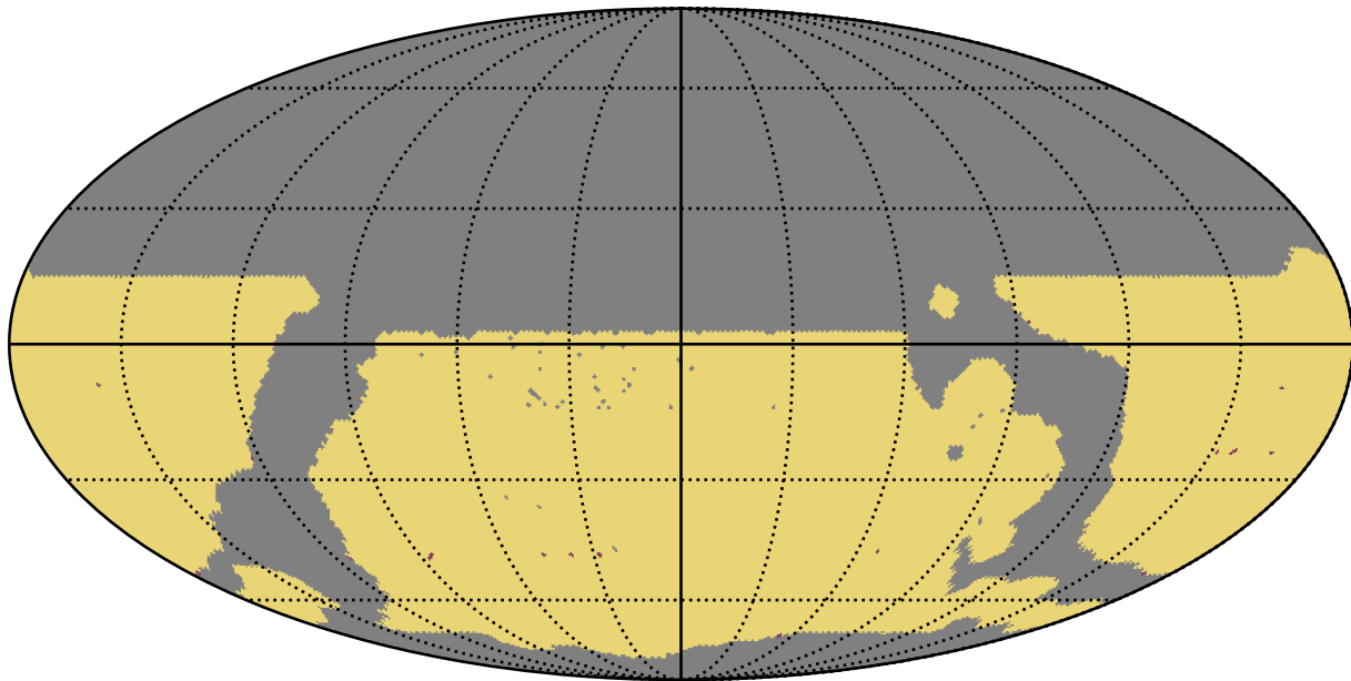
weather_cloudso35v3.4_10yrs WFD: RapidRevisits
