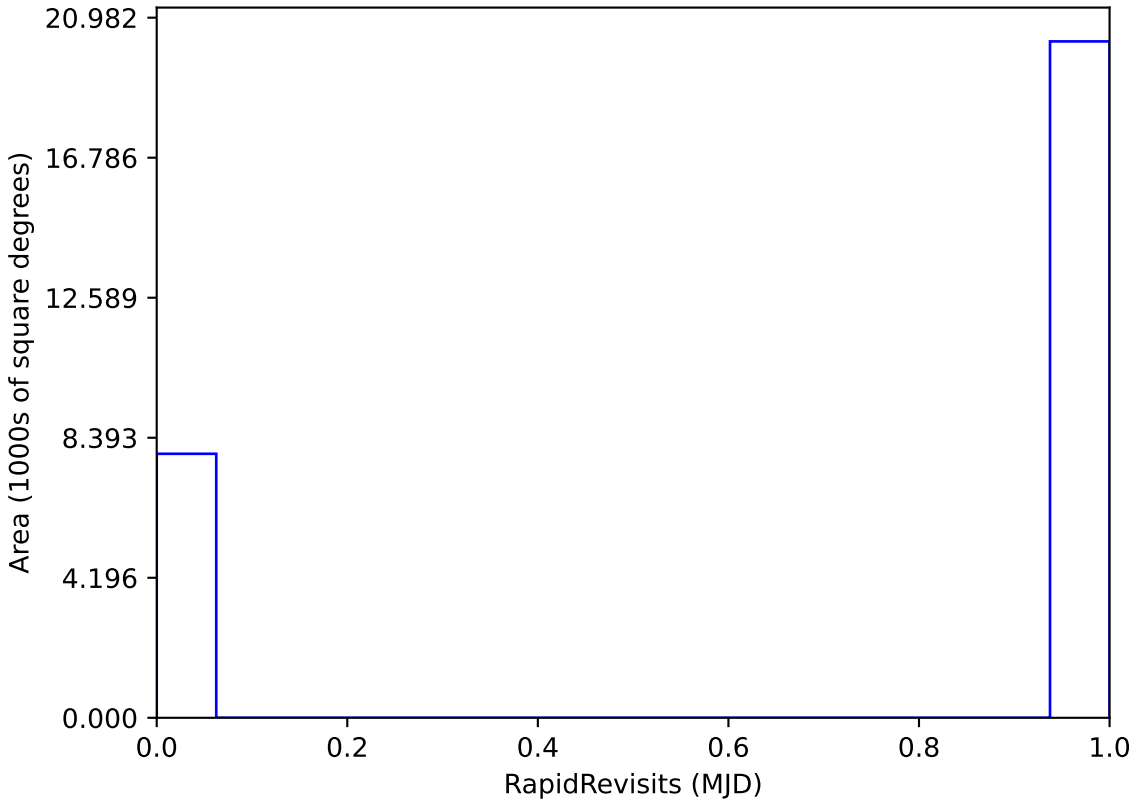
weather_cloudso35v3.4_10yrs All sky: RapidRevisits
